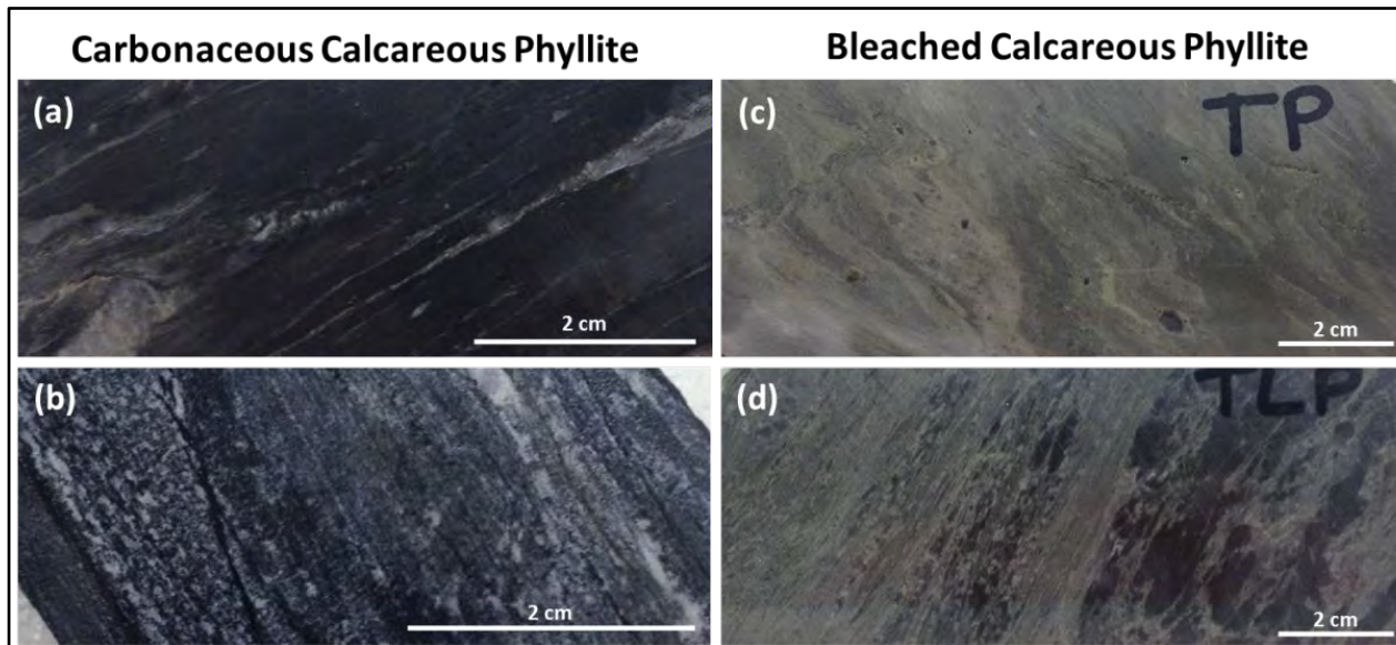
Figure 7-3: Typical Phyllites of the Bornite Carbonate Sequence
