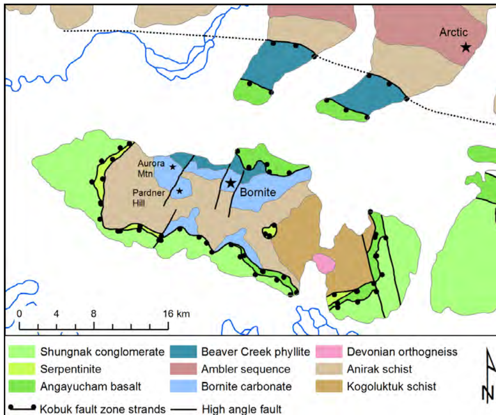
Figure 7-1: Generalized Geologic Map of the Local Geology
